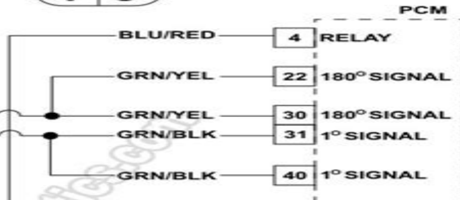
CRANK ANGLE SENSOR CONNECTOR ON DISTRIBUTOR
