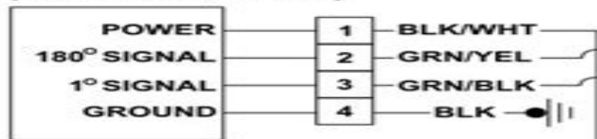
CRANK ANGLE SENSOR (INSIDE DISTRIBUTOR)
