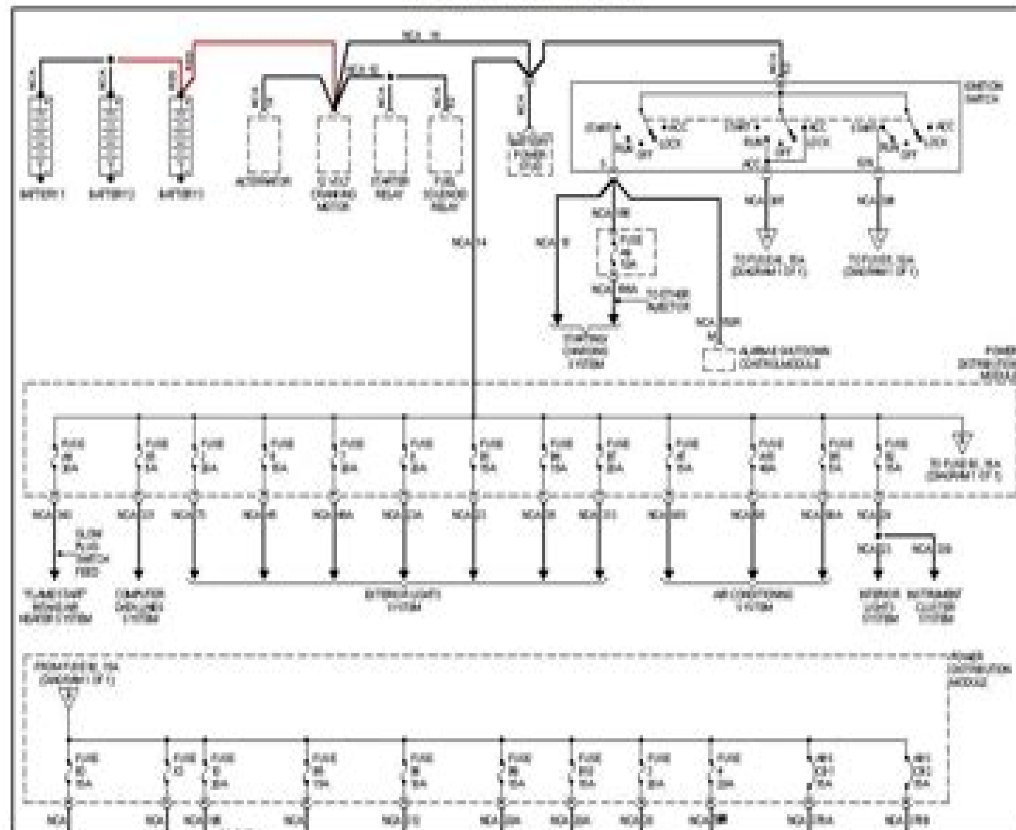
Fig. 31: Power Distribution Circuit
