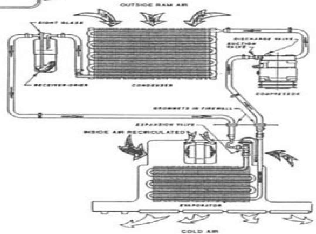
AUTO AIR CONDITIONING REFRIGERANT CYCLE
