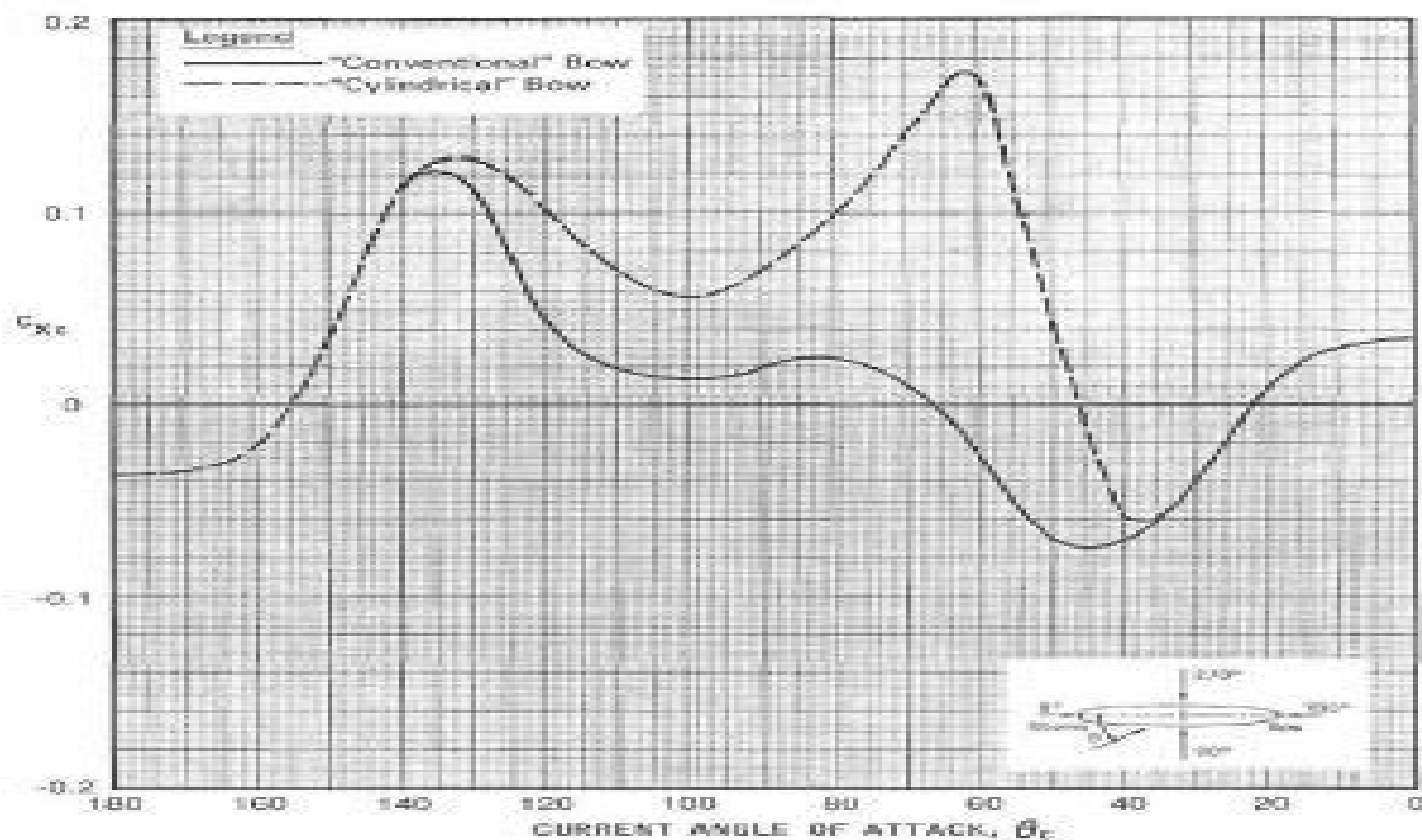
FIGURE 7 LONGITUDINAL CURRENT FORCE COEFFICIENT-LOADED TANKER ( W/D = 1.5 )
