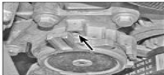
21.10 Insert a 5.0 mm drill bit/rod into the hole (arrowed) in the tensioner housing
