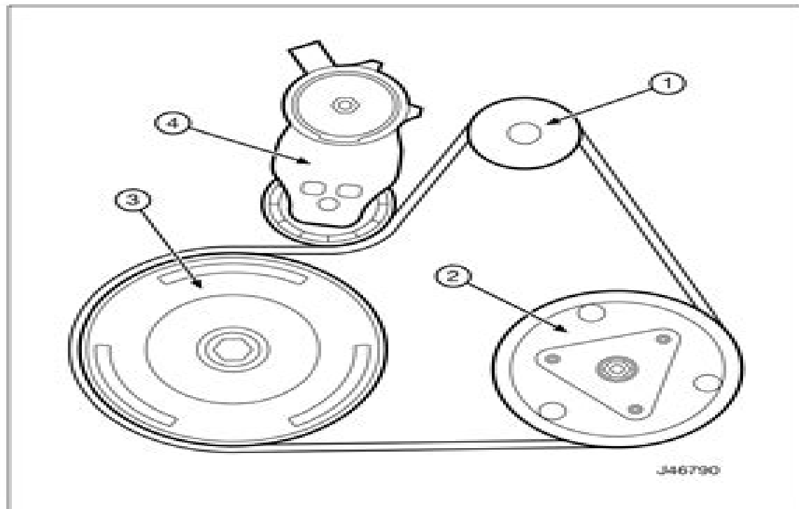
21.11 Auxiliary belt routing
