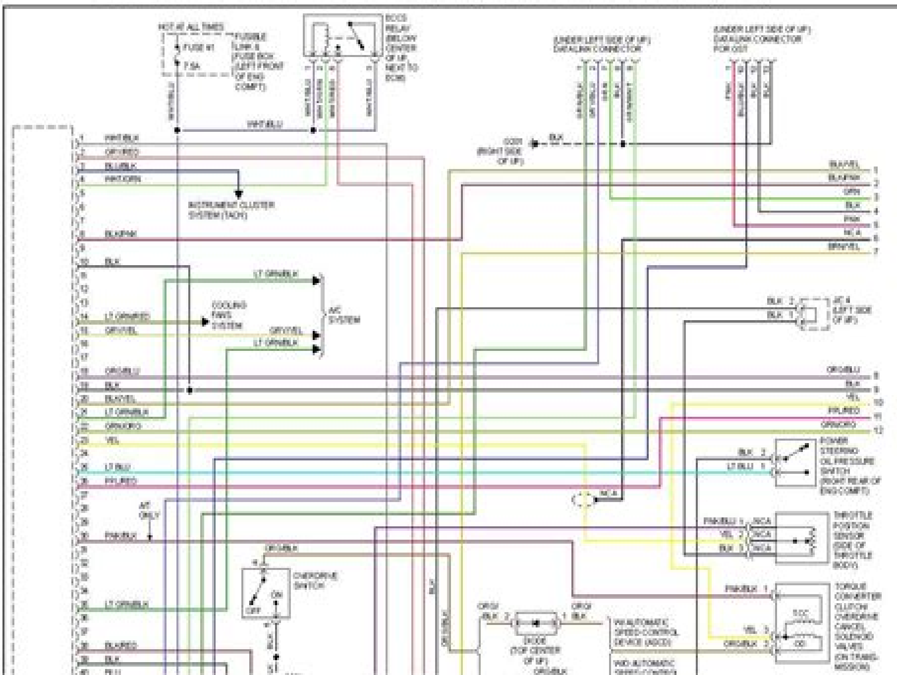
1995 Nissan Sentra GXE-Fig. 13: 1.6L, Engine Performance Circuits (1 of 2)
