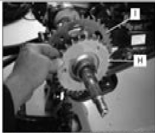
9. Remove the 30 tooth sprocket (H) and the 38 tooth sprocket (I).
