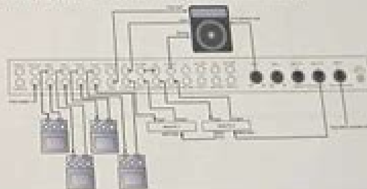
Diagram 2: Four 1/4" Inputs, Two Amps
