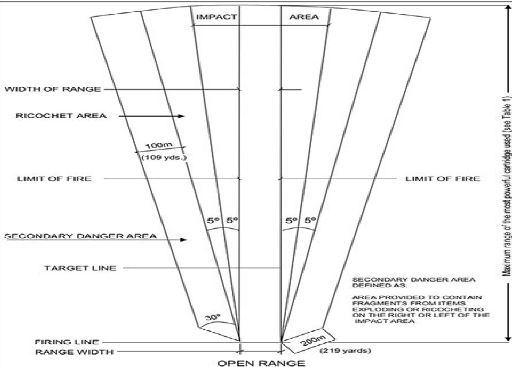
Figure 1 Surface Danger Zone for Small Arms Firing at Fixed Ground Targets
