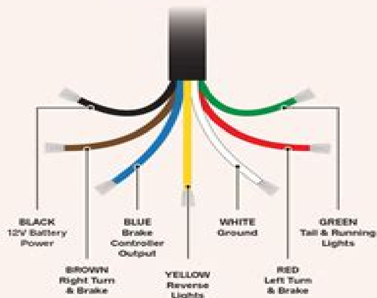
Wiring Side
