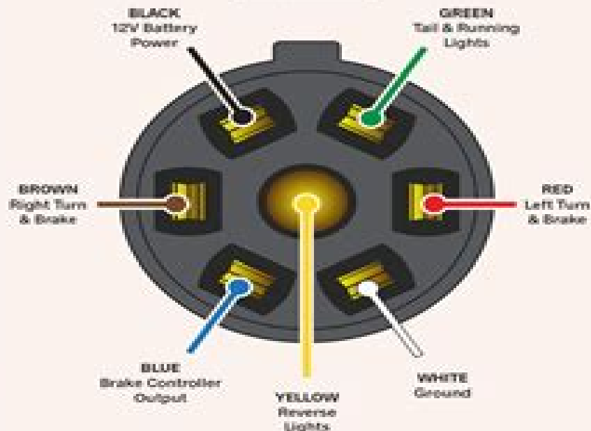
Plug Side
