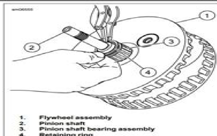
Figure 3-91. Removing Pinion Shaft Bearing Retaining Ring
