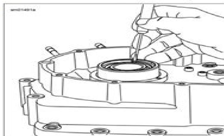
Figure 3-92. Removing Left Main Oil Seal Retaining Ring
