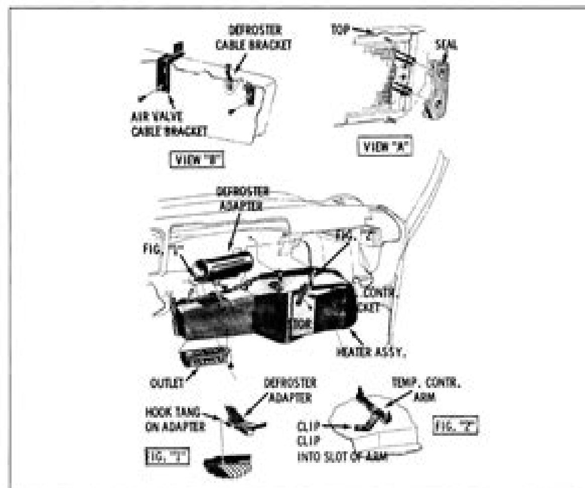
Fig. 1-15—Heater Assembly
