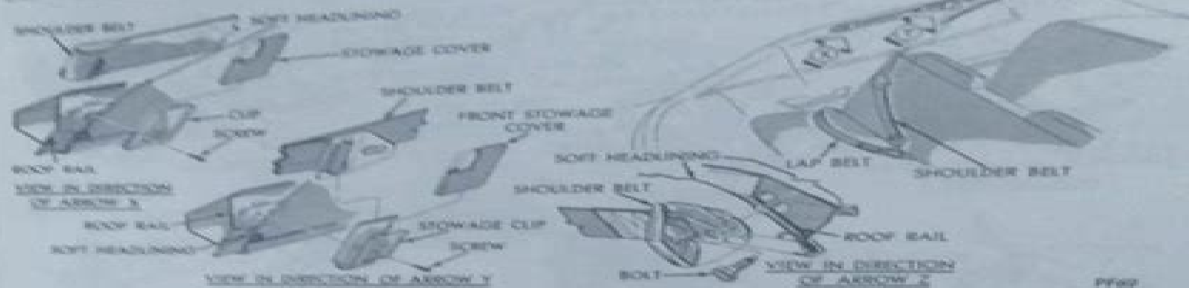
Fig. 20—Front Seat Shoulder Belt (J)
