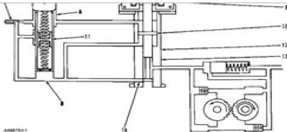
SCHEMATIC OF PSG GOVERNOR.
