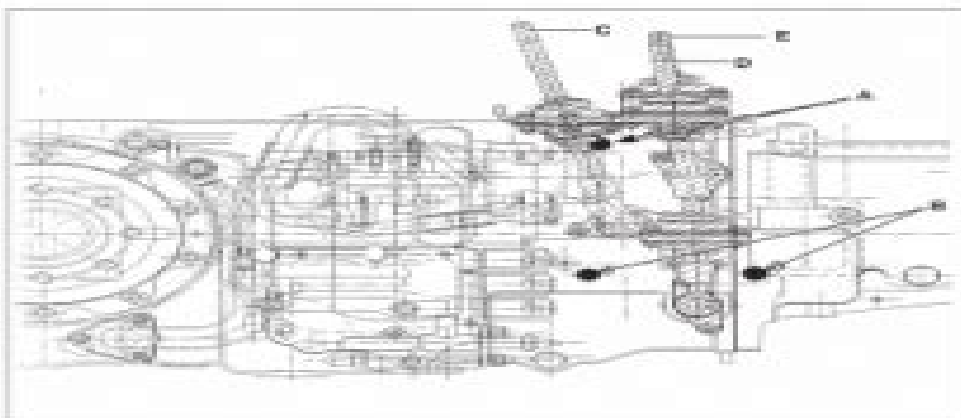
Fig. 16 - Retaining screws of the gear rods to be removed prior to detaching the front gearbox from the rear gearbox.
