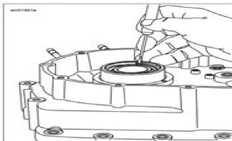
Figure 3-92. Removing Left Main Oil Seal Retaining Ring
