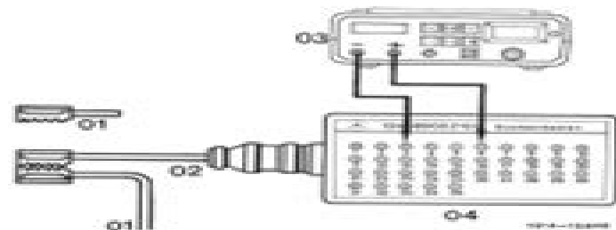
Fig. 91/17 Connection diagram socket box
