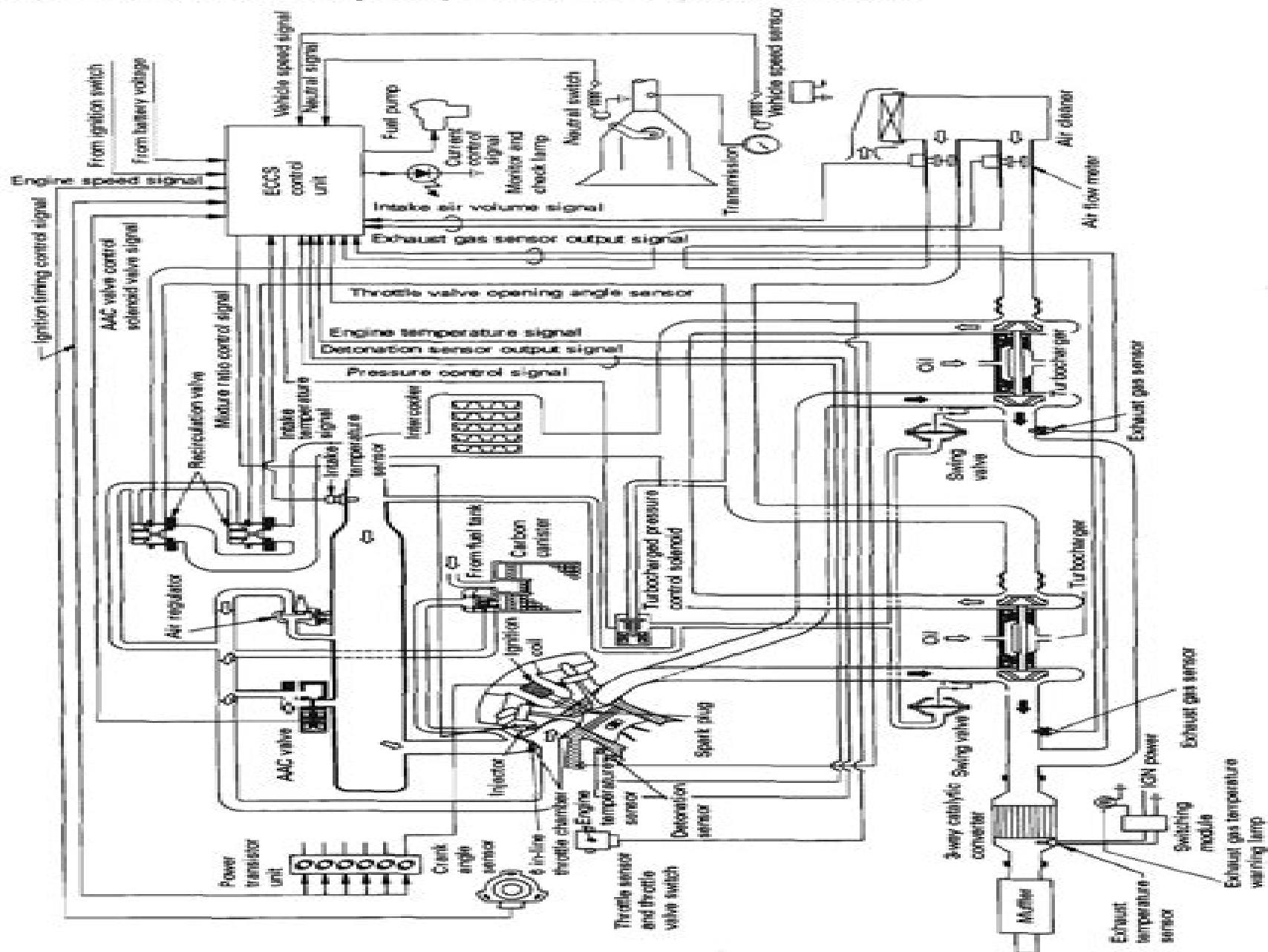
3-1 RB26 DOHC — EGI (ECCS) TWIN-TURBOCHARGER ENGINE
