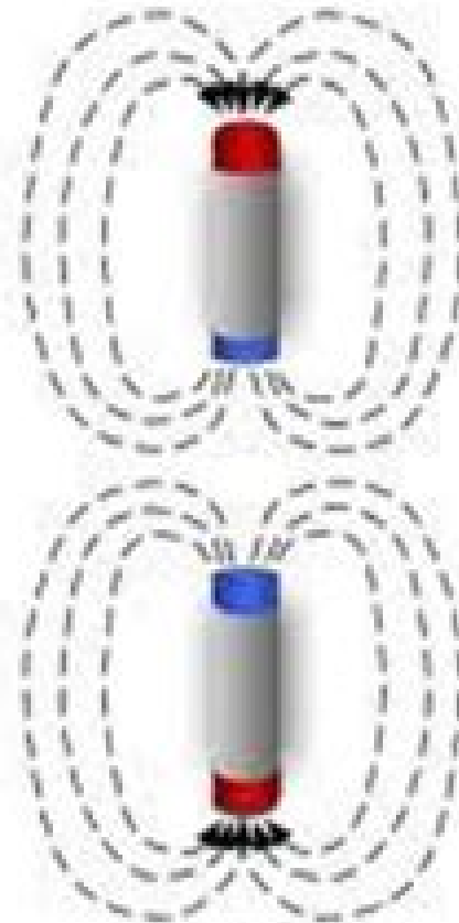
Magnetic Repulsion (conventional view)
