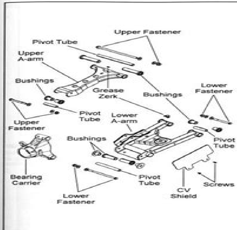
Exploded View (RZR)
