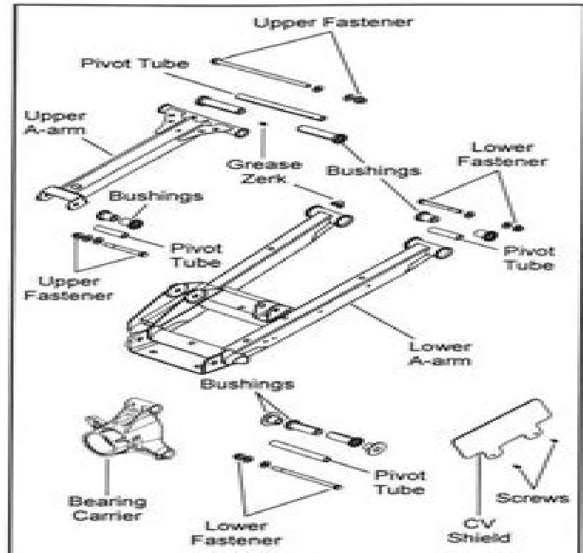
Exploded View (RZR S / RZR 4)
