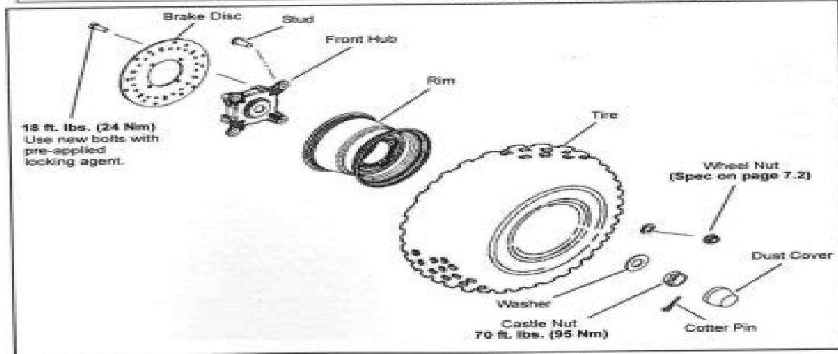
Front Hub/Wheel Exploded View
