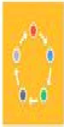
Team Development
