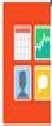
Packaged Apps
