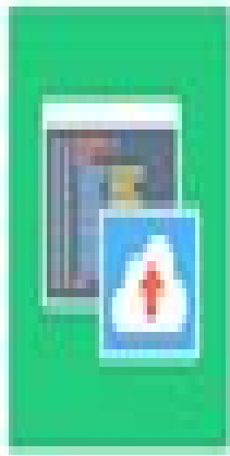
SQL Workshop
