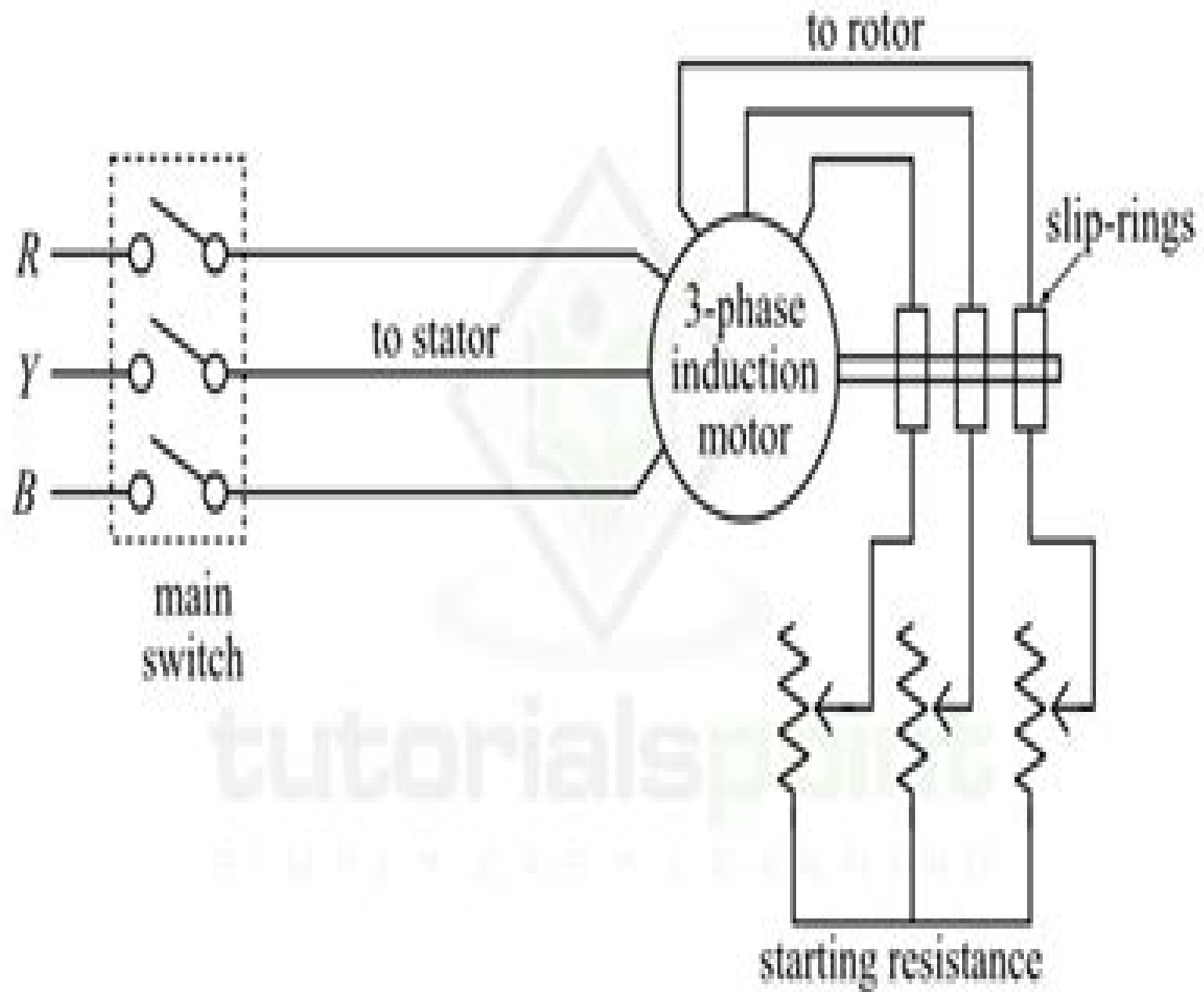
Figure 4 - Rotor Resistance Starter
