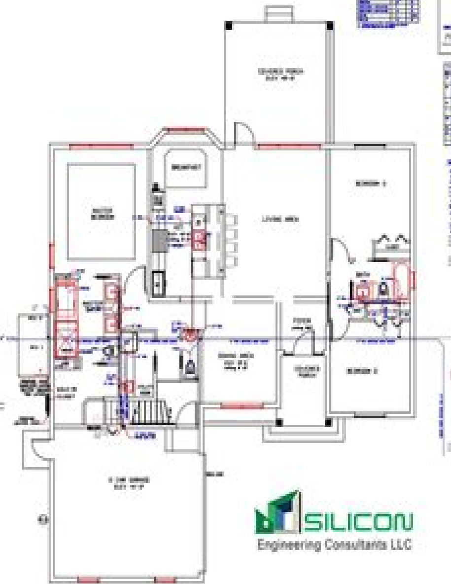
GROUND FLOOR PLAN (DRAINAGE & WATER SUPPLY) 1/4" = 1'-0"
