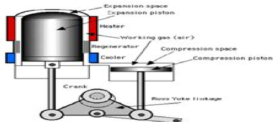
Fig. 1. Stirling engine [2]
