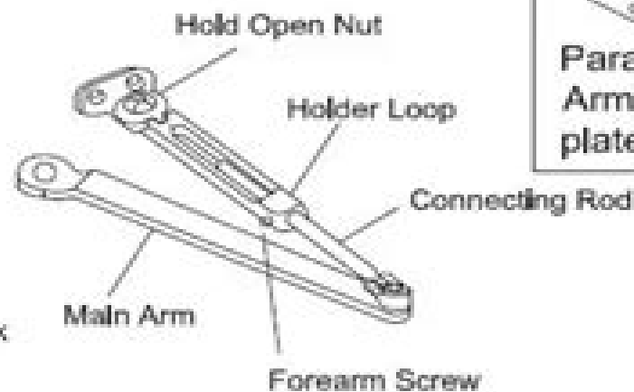
Closer Arm
