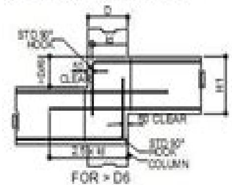
STEPPED BEAM COLUMN CONNECTION
