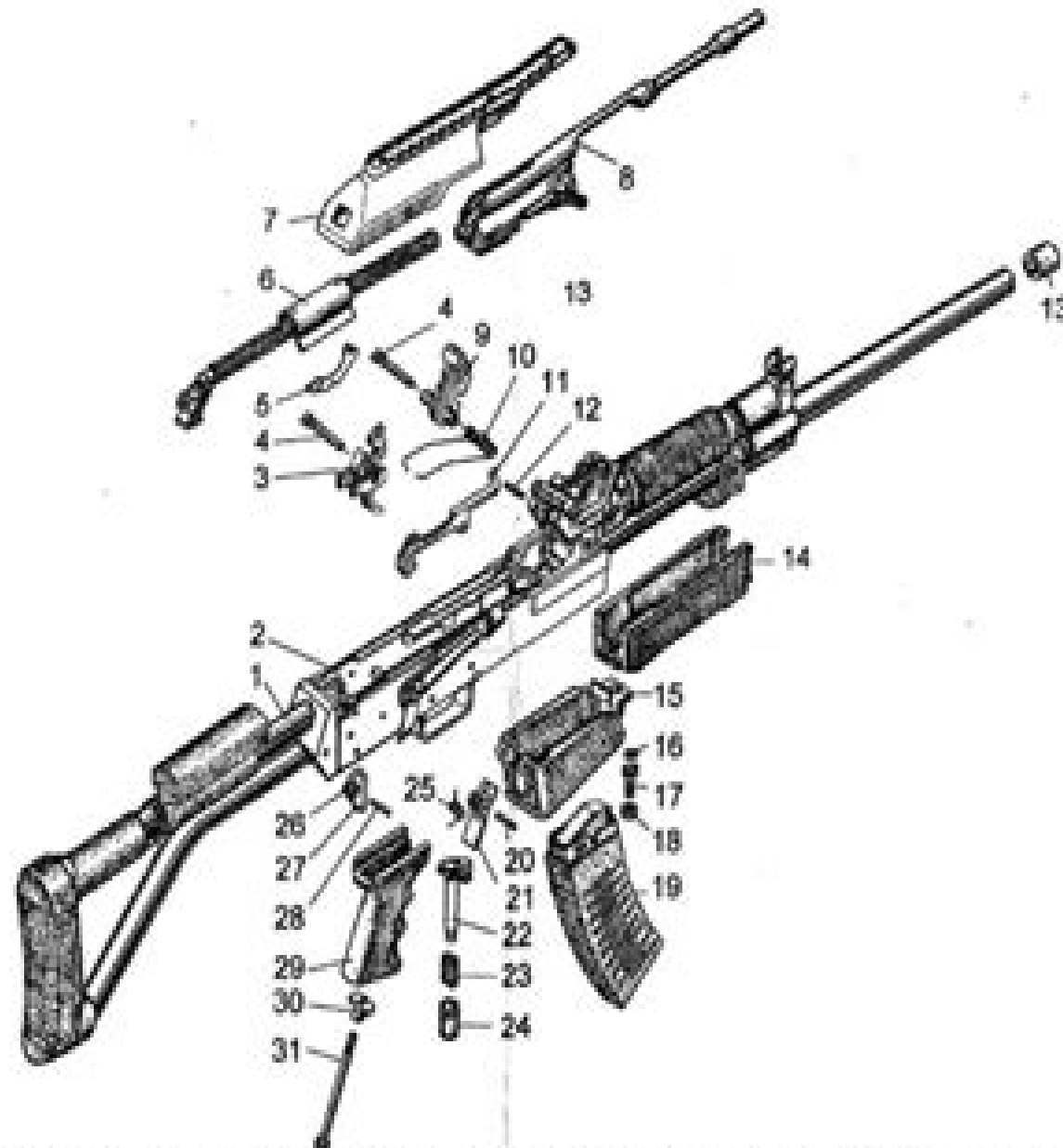
1- butt; 2-receiver with barrel; 3-rigger mechanism; 4-axis of trigger mechanism; 5-detent; 6-recoil mechanism; 7-cover; 8-bolt carrier with bolt; 9-hammer; 10-mainspring; 11-lever; 12-pin; 13-nut; 14- forearm; 15-feed block; 16-washer; 17-bolt; 18-nut; 19-magazine; 20-magazine-catch pin; 21-magazine catch; 22-bolt stop; 23-spring; 24-nut; 25-catch spring; 26-swivel base; 27- swivel ring; 28-axis of swivel; 29-grip; 30- nut; 31- coupling screw.
