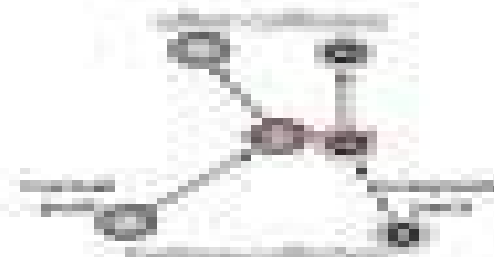
Figure 1. uncollided two parts of an elastic collision force.
