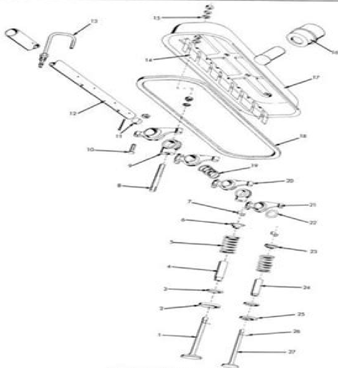
VALVES & ROCKER ARMS Gasoline & LPG
