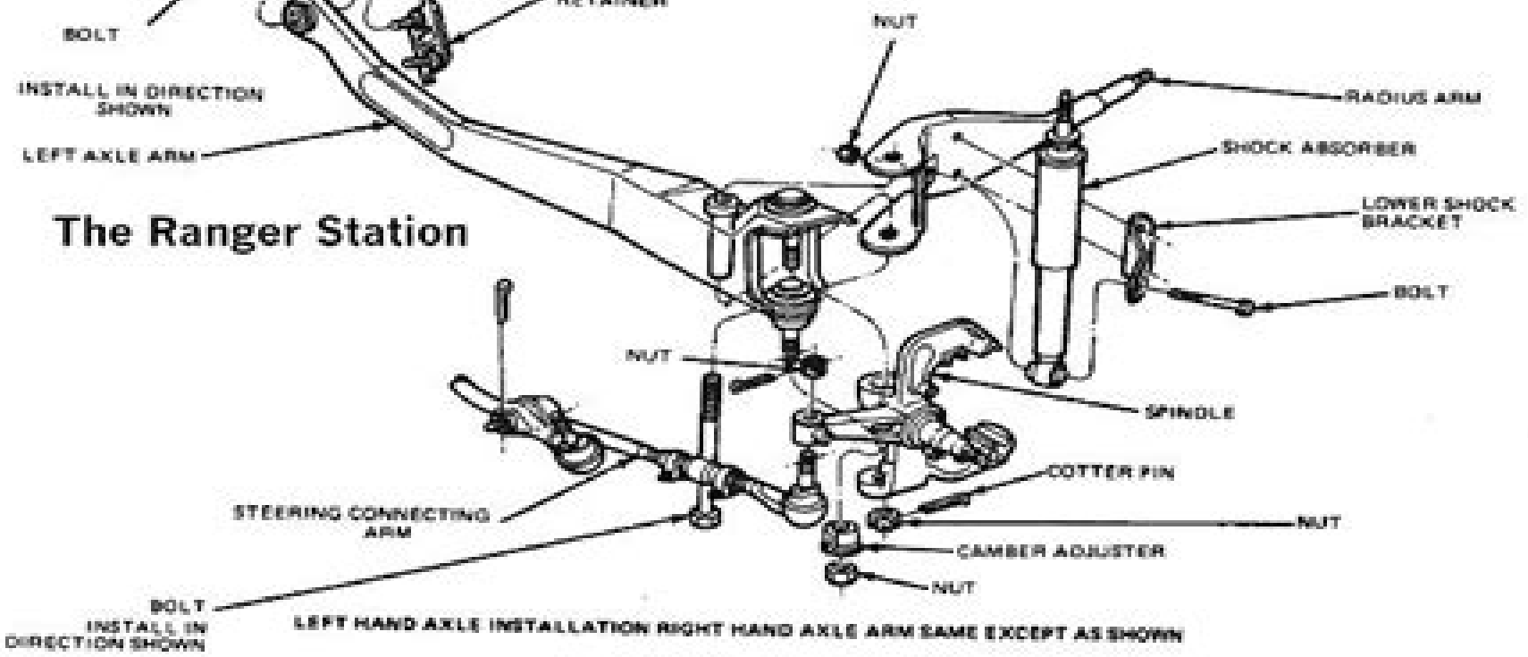
An exploded view of the radius arm and related parts (2WD models) (1983 through 1992 models shown, 1993 models similar)
