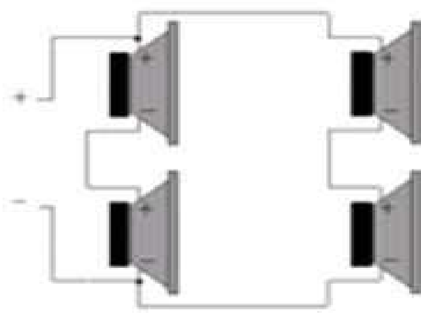
Wiring Four Speakers in Series
