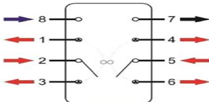
CIRCUIT DIAGRAM
