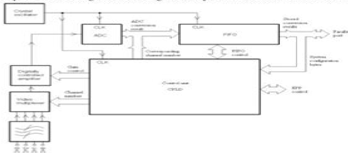
Figure 2. Blockdiagram of the digitizer
