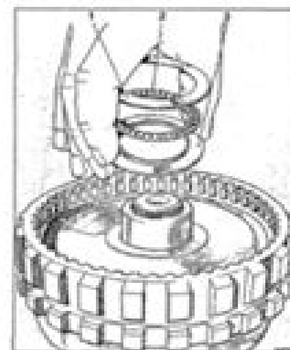
Fig. 11B-16 Fitting the rear and thrust bearing to the outer face of the rear internal gear 1. 5/16 tapered nut 2. Thrust bearing 3. 1/2 tapered nut
