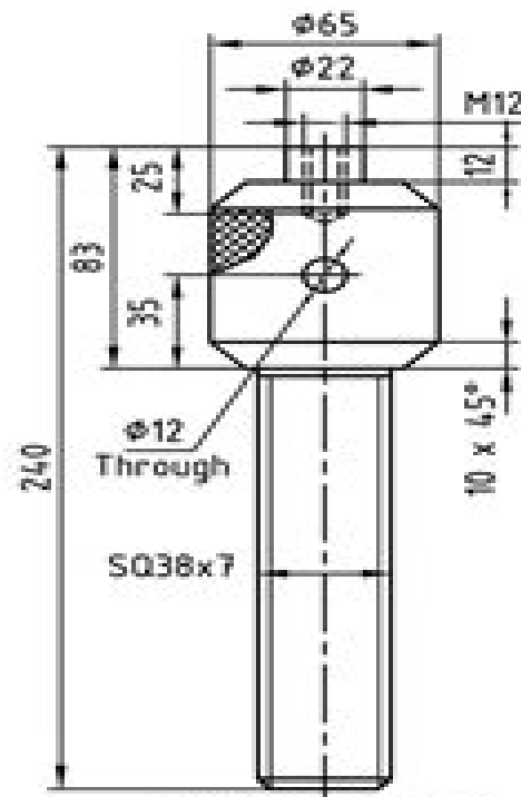
SCREW SPINDLE (MILD STEEL)
