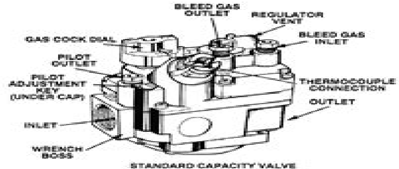
STANDARD CAPACITY VALVE
