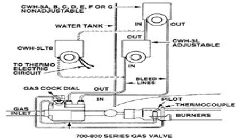
700-800 SERIES GAS VALVE
