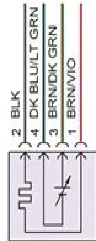
OXYGEN SENSOR 2/1
