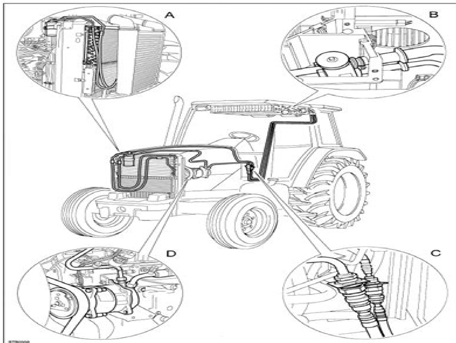
Air Conditioning Component Layout
