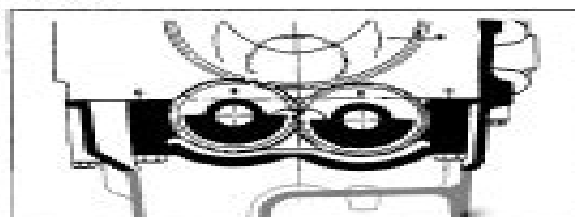
Fig. 38 - Counterbalance weights assembly.
