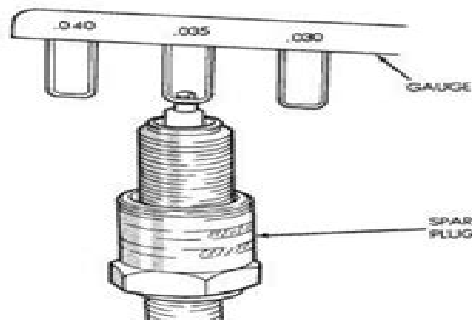
Fig. 6 Setting Spark Plug Electrode Gap—Typical
