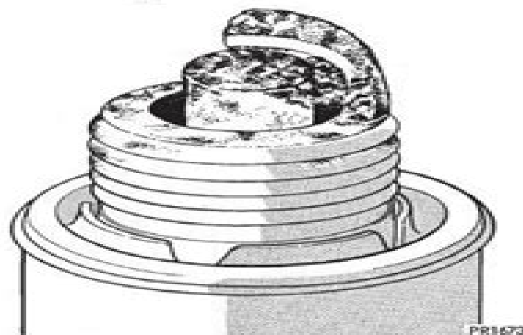
Fig. 8 Oil or Ash Encrusted
