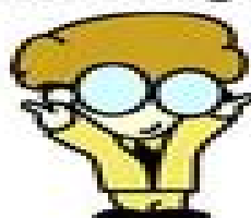
Seismologist
