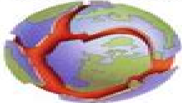
Convection
