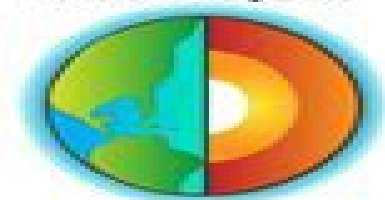
Earth Layers
