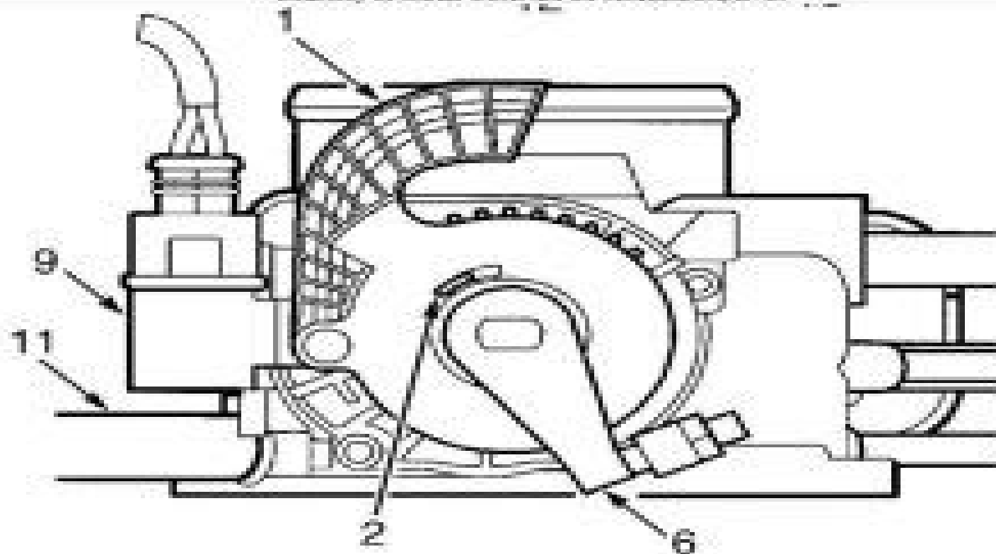
Fig. 17: Identifying 4-Cylinder Throttle Body Components
