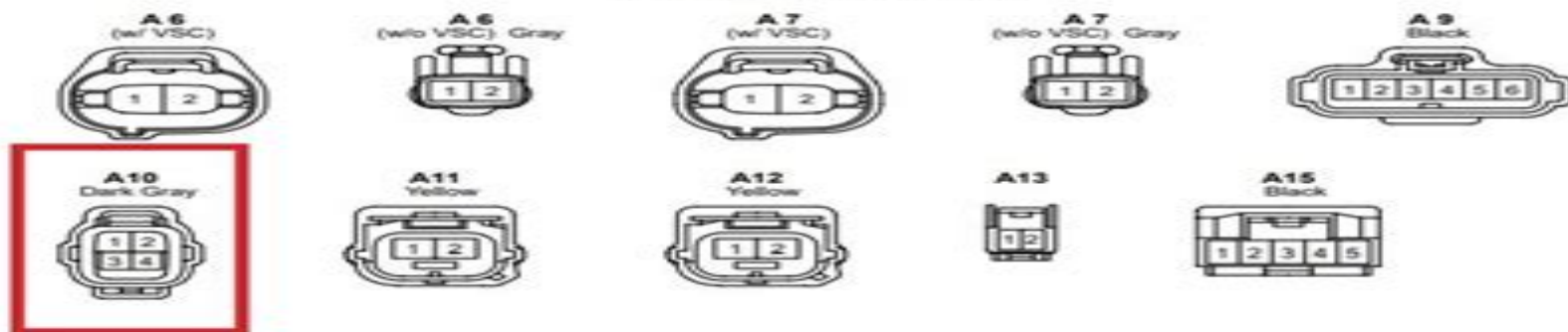
2005 TOYOTA TUNDRA (EWD611U)
