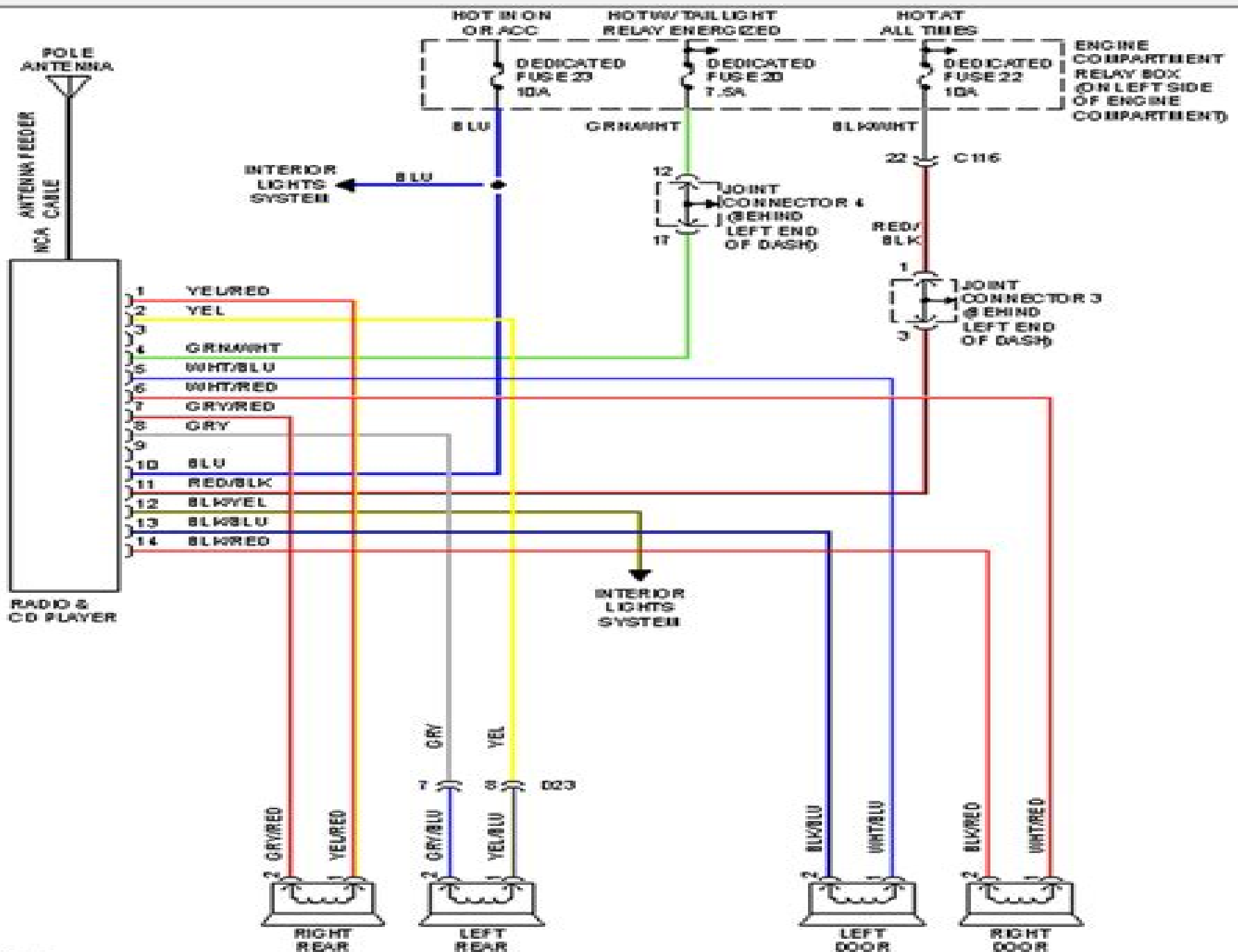
Fig. 39: Radio Circuit, W/D Amplifier
