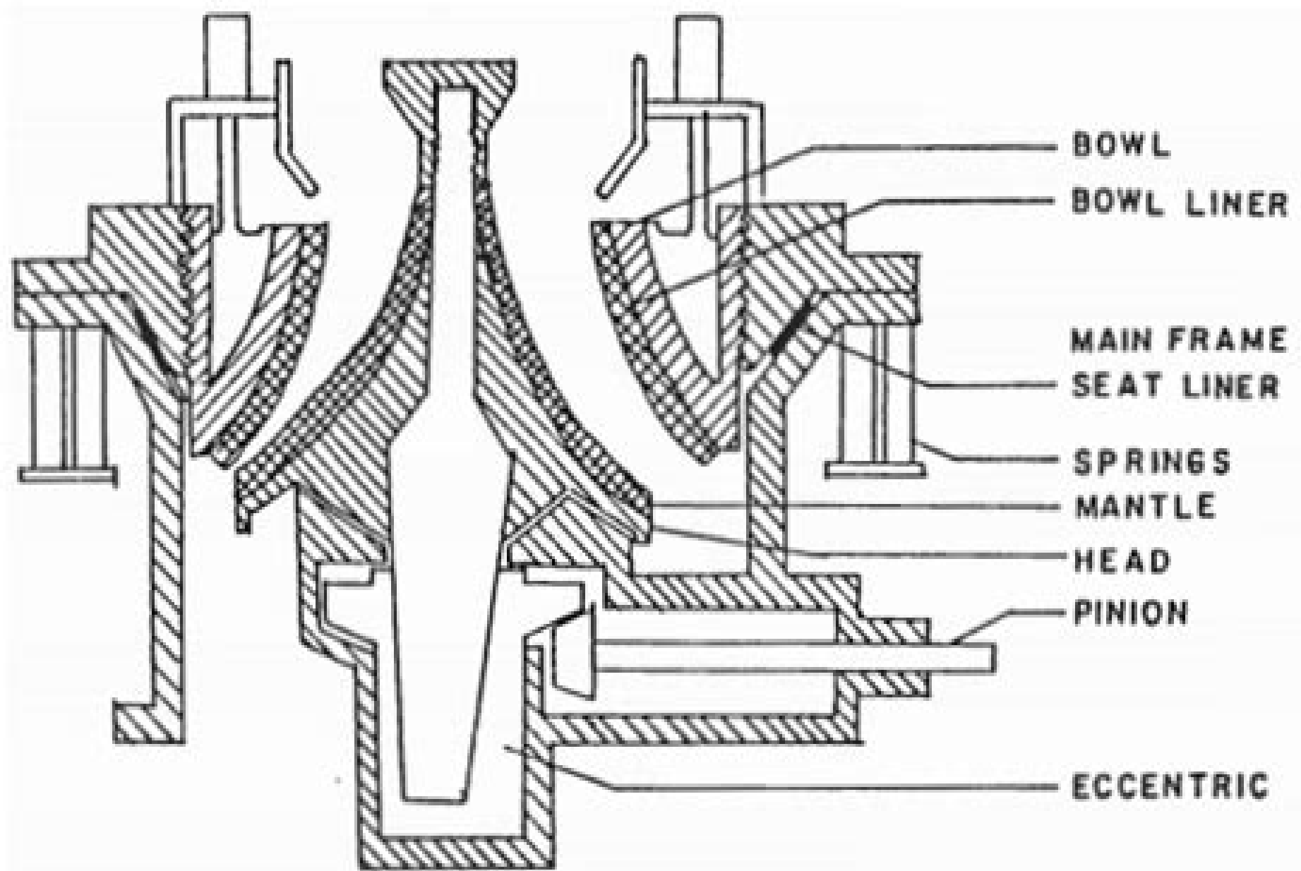
SYMONS / SPRING CONE CRUSHER
