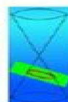
Ellipse
