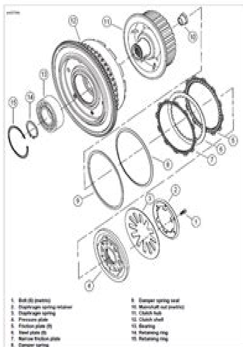
Figure 5-29 Clutch Shaft Assembly
