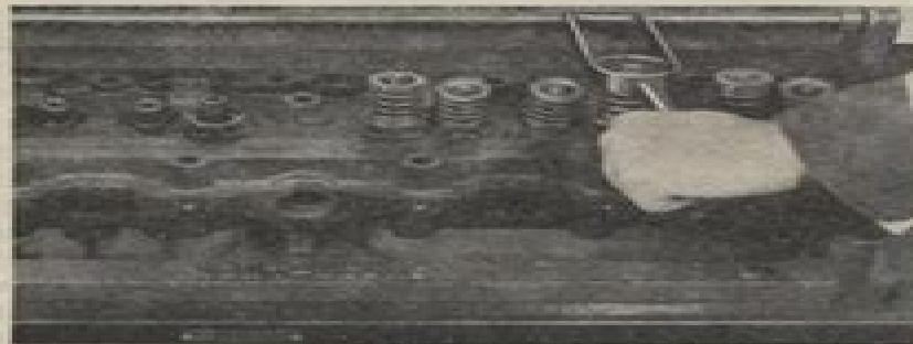
Fig. 71—Valve Spring Compressor
