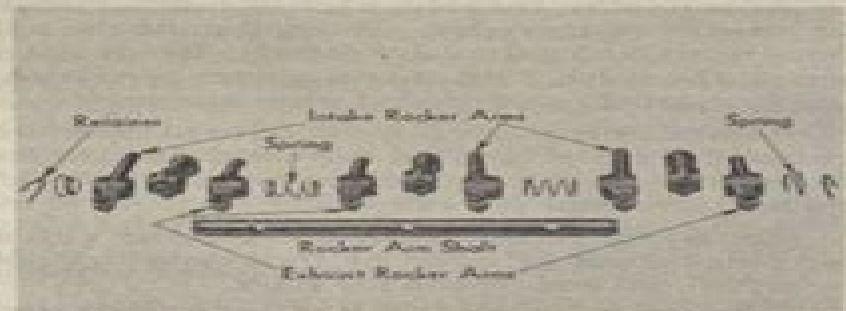
Fig. 74—Rocker Arm and Shafts
