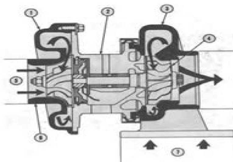
Figure 1 Turbocharger Air Flow
